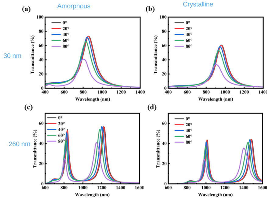
Fig. 4. The simulation transmission spectra of the multilayer film under different incident angles for Sb 2 Se 3 thicknesses of 30 nm and 260 nm: (a) amorphous and (b) crystalline states at 30 nm; (c) amorphous and (d) crystalline states at 260 nm.
